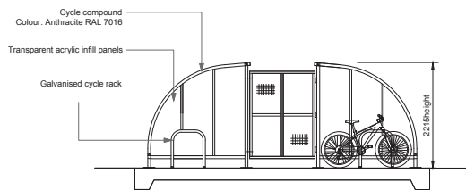
Cycle Shelter Section A-A
