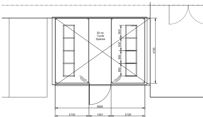
Cycle Shelter Key Plan
