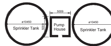
Sprinkler Tanks and Pump House Plan
