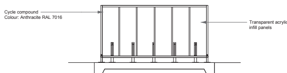
Cycle Shelter Elevation C
