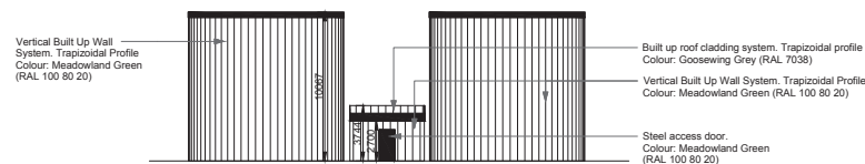
Sprinkler Tanks and Pump House Elevation D
