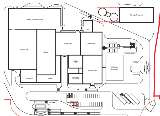
Site Key Plan
