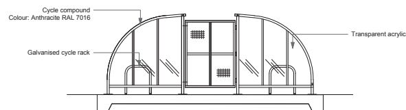
Cycle Shelter Section B-B
