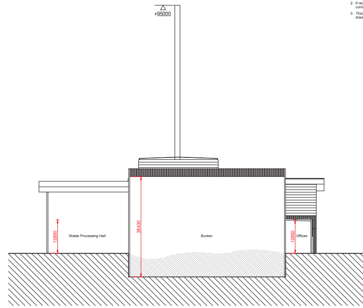
Section B-B 1:500
