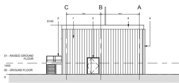
2 West Elevation 1 : 100
