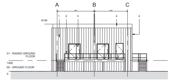
4 East Elevation 1 : 100
