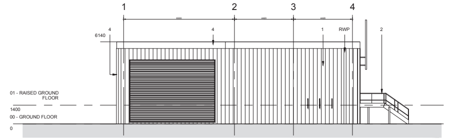
3 South Elevation 1 : 100
