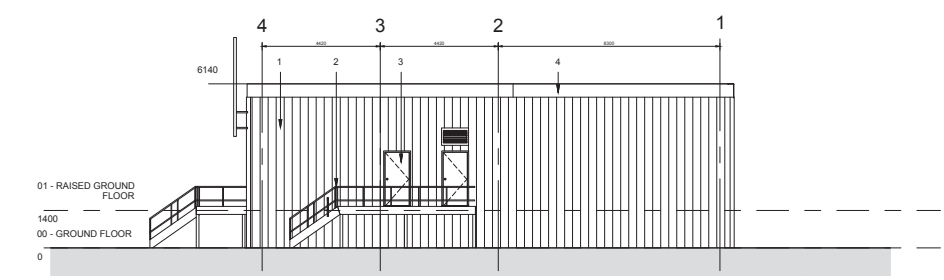
1 North Elevation 1 : 100
