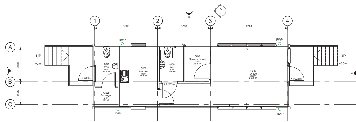
Gatehouse Floor Plan 1 : 50
