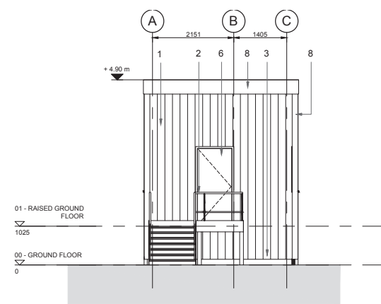
West Elevation 1 : 50
