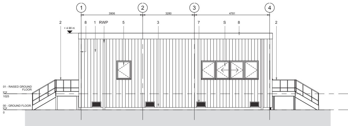
North Elevation 1 : 50
