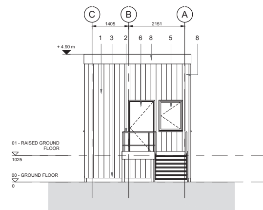
East Elevation 1 : 50
