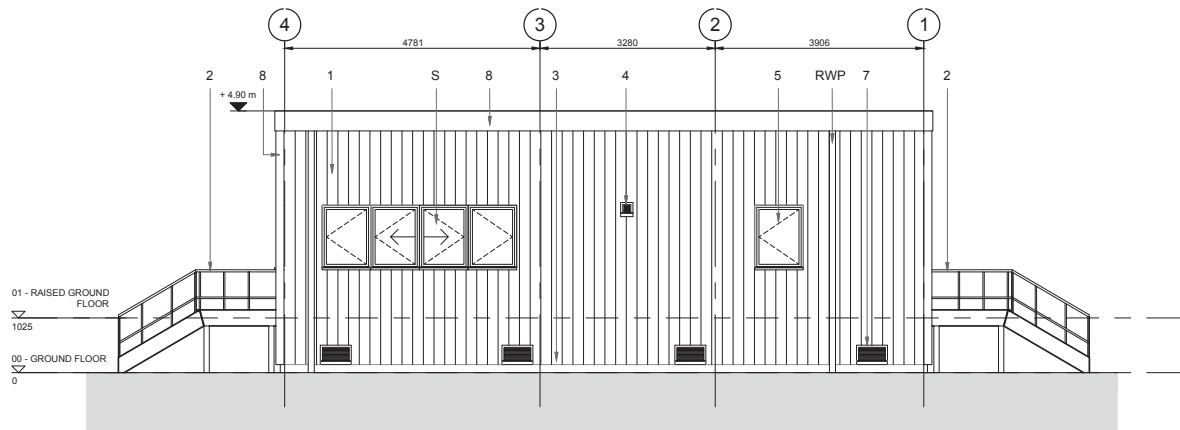
South Elevation 1 : 50
