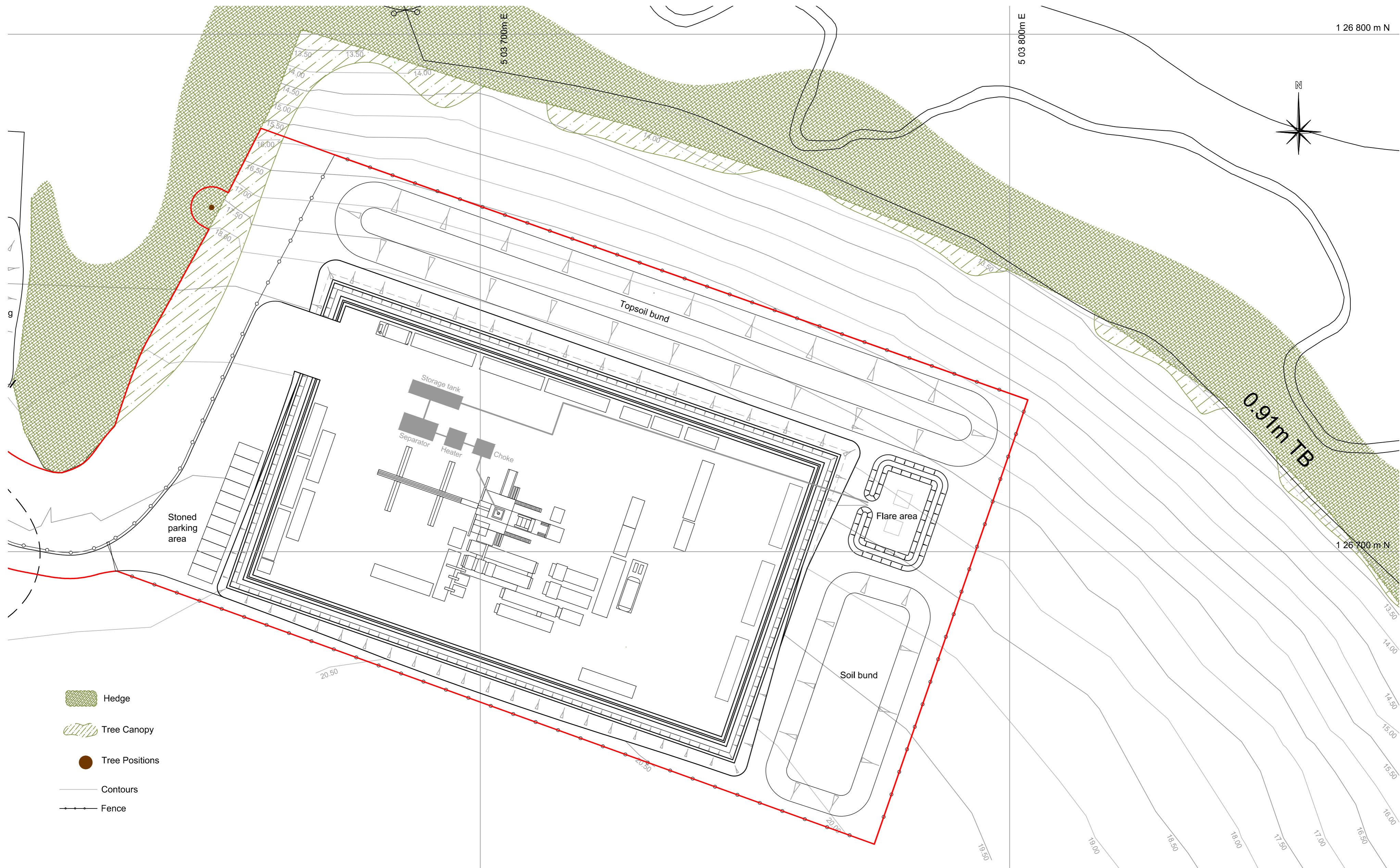
Proposed Site - Drill Stem Testing Mode Scale 1:500
