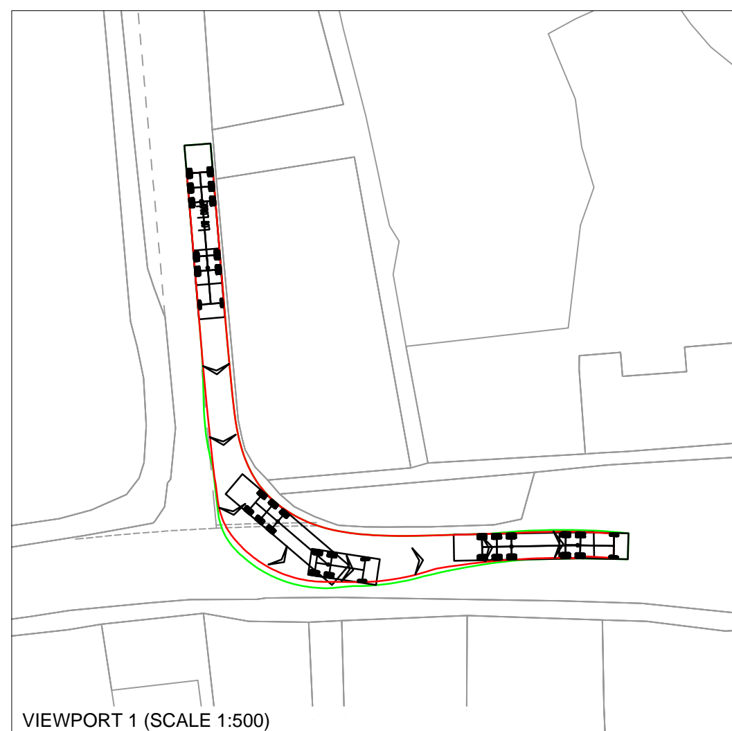
VIEWPORT 1 (SCALE 1:500)
