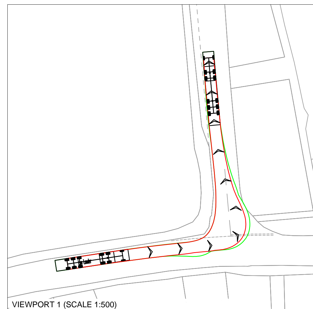
VIEWPORT 1 (SCALE 1:500)
