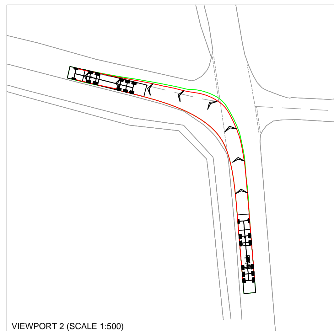
VIEWPORT 2 (SCALE 1:500)
