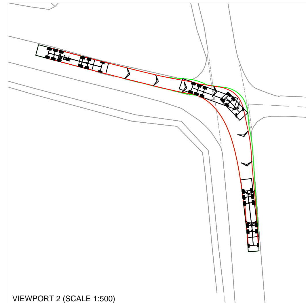
VIEWPORT 2 (SCALE 1:500)
