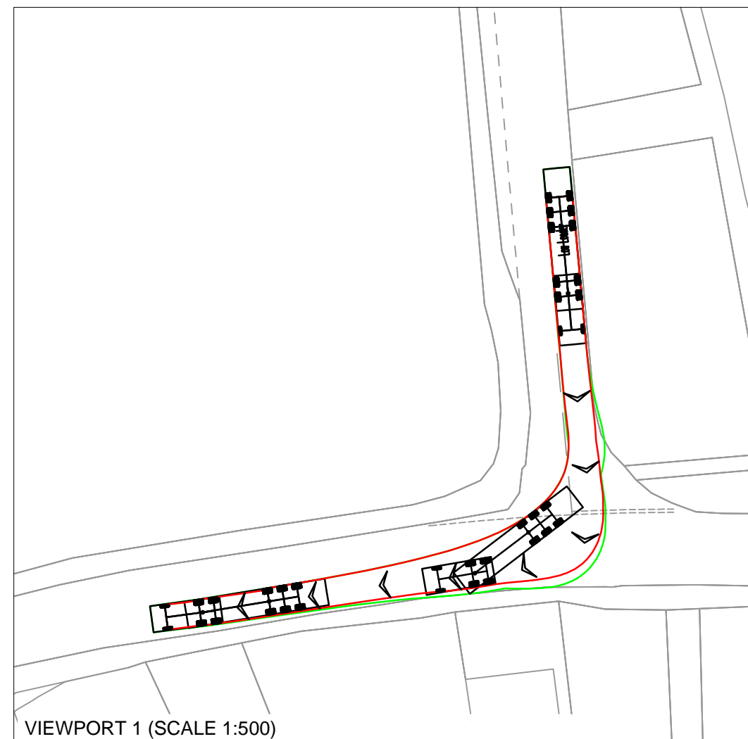
VIEWPORT 1 (SCALE 1:500)
