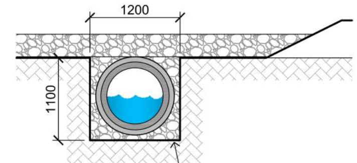
750mm ID concrete pipe covered with 300mm site stone COVERED PIPE DITCH
