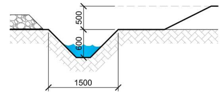
STANDARD 'V' DITCH
