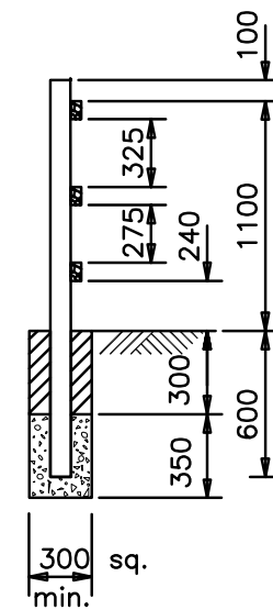
SECTION THROUGH C OF MAIN POSTS
