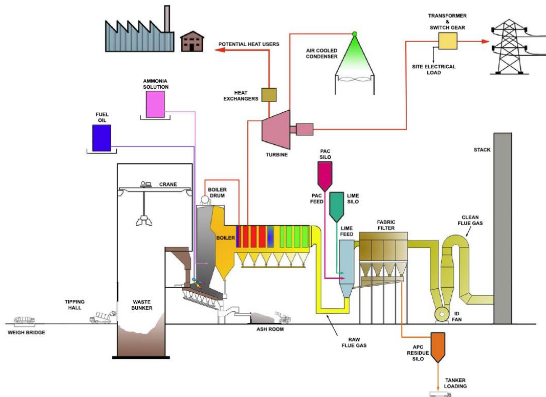
Figure 2: Process schematic
