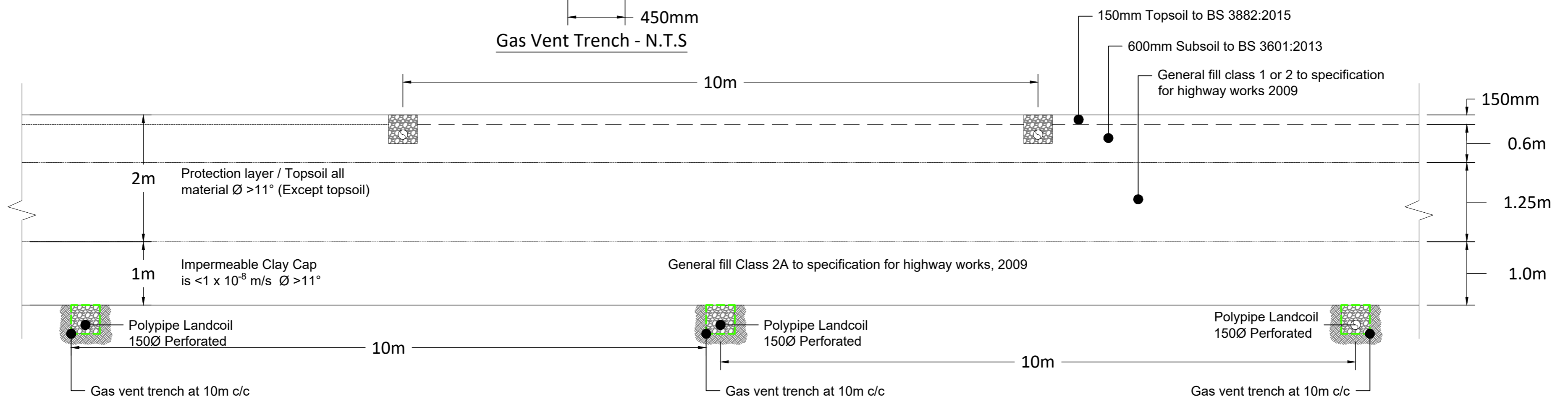
Section of capping layer - shallow slopes
