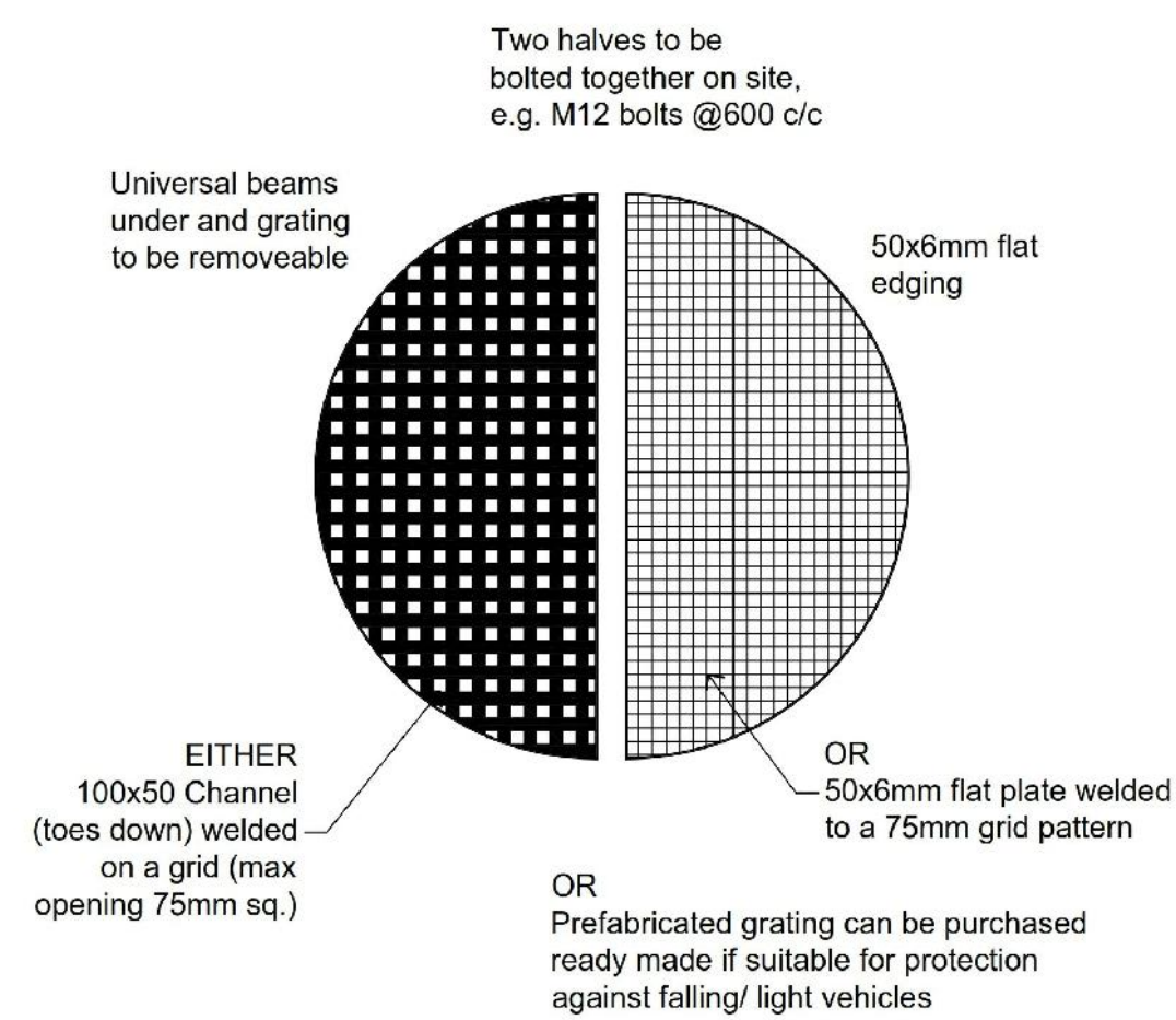
CELLAR GRATING DETAIL Scale 1:50
