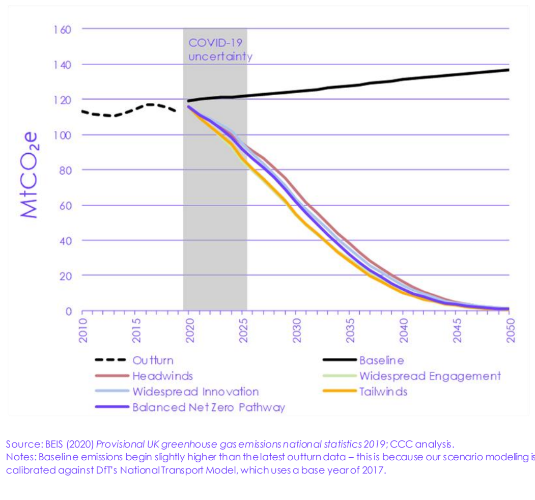
Figure 3.1.c Emissions pathways for the surface transport sector
