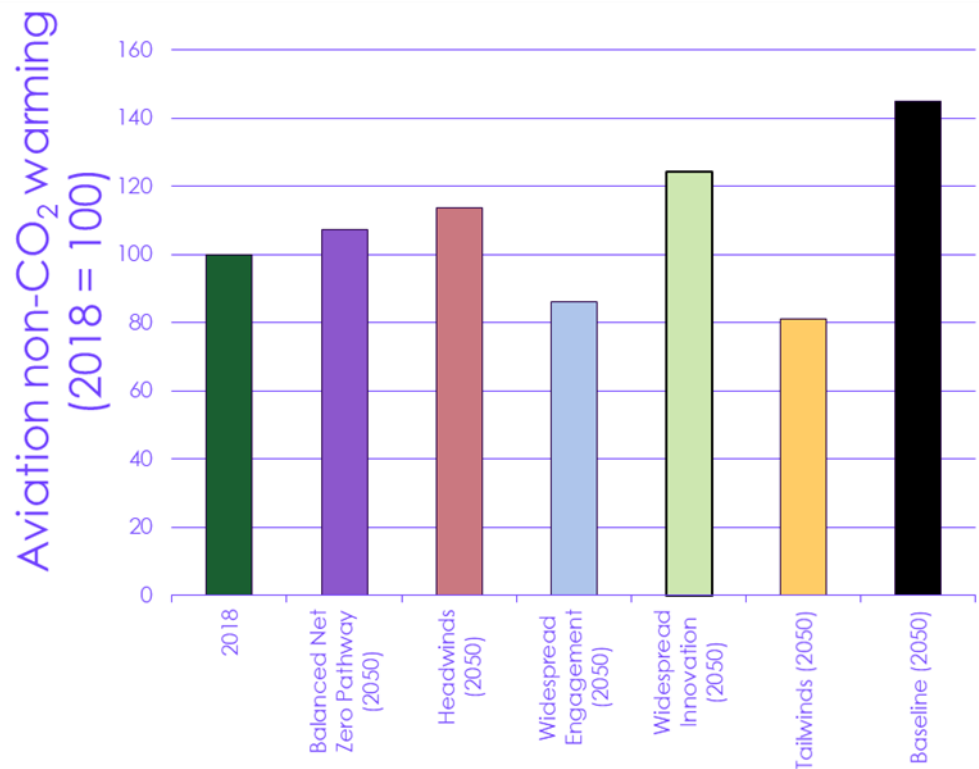
Figure B8.7 Warming from UK non-CO 2 aviation effects in 2050 relative to 2018
