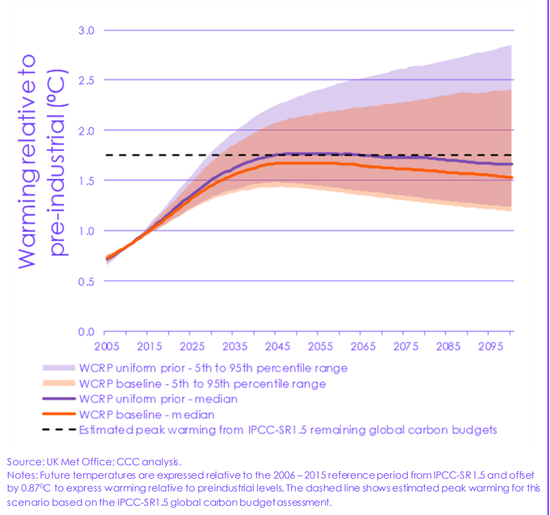
Figure 8.3 Global temperature projections under WCRP climate sensitivity distributions for a rapid global decarbonisation scenario
