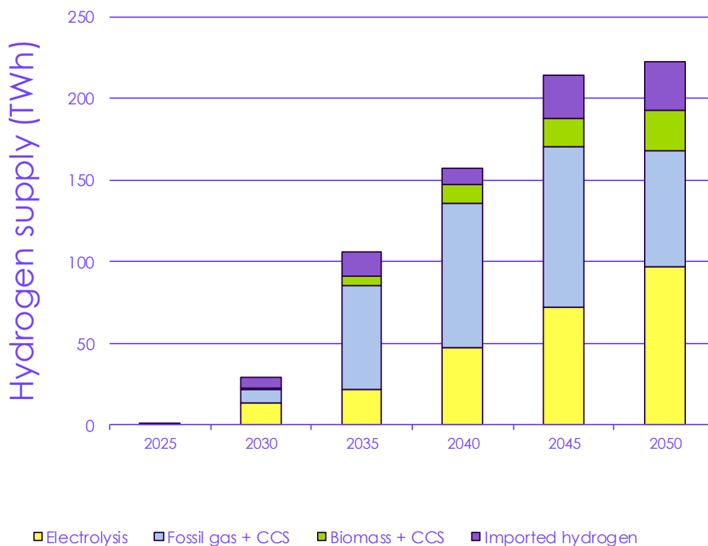
Figure 3.5.c Hydrogen supply in the Balanced Net Zero Pathway
