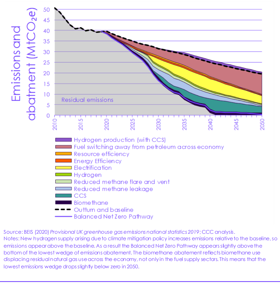
Figure 3.5.a Sources of abatement in the Balanced Net Zero Pathway for the fuel supply sector
