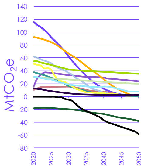
Figure 5 Sectoral emissions under the Balanced Net Zero Pathway
