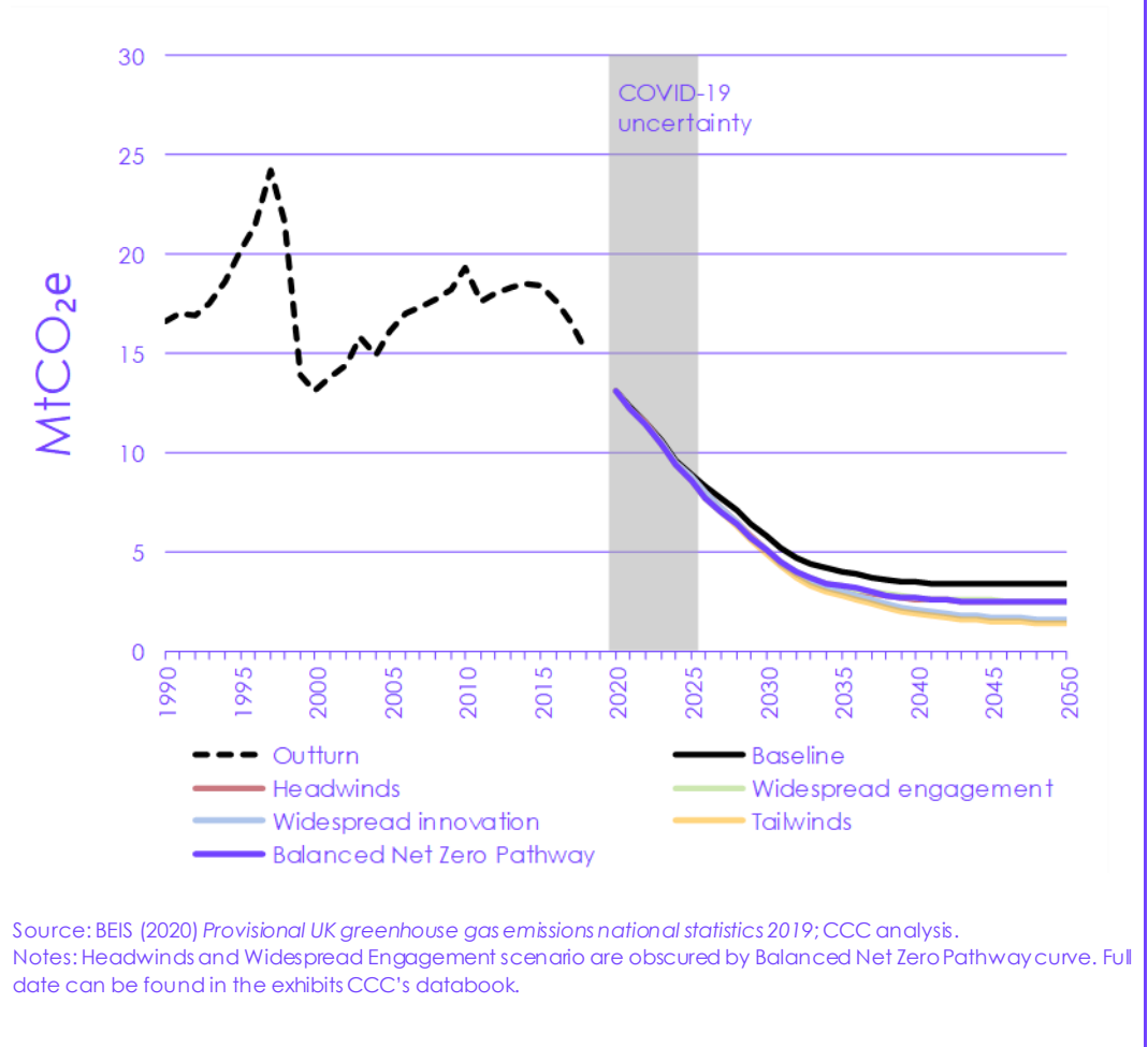
Figure 3.10.a Emissions pathways for the F-gases sector
